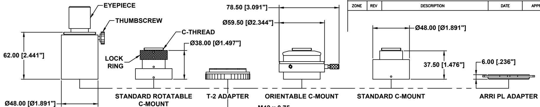
M62 EYEPIECE HOLDER TUBE & EYEPIECE
