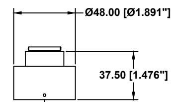
STANDARD C-MOUNT
